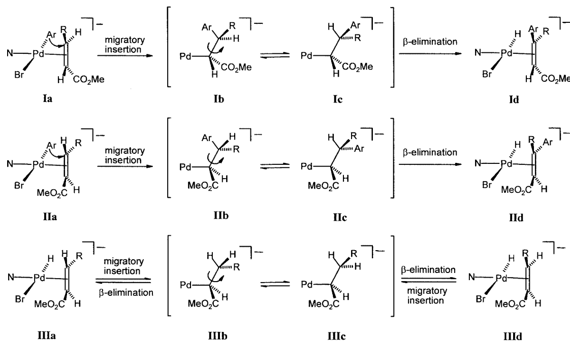
Scheme 6. Mechanistic scheme representing the stereospecific migratory insertion- \beta -elimination sequence in the Heck reaction involving 1,2-disubstituted alkenes
