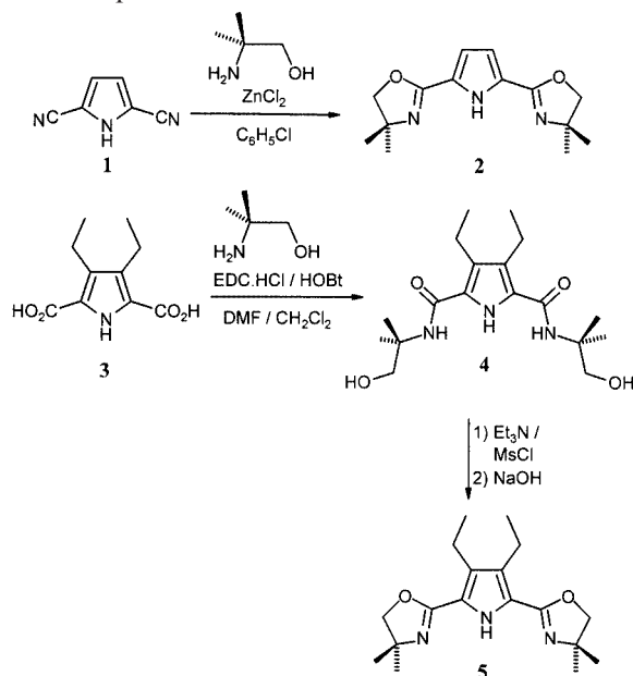
Scheme 1. Synthesis of the two bis(oxazolinyl)pyrroles 2 and 5
