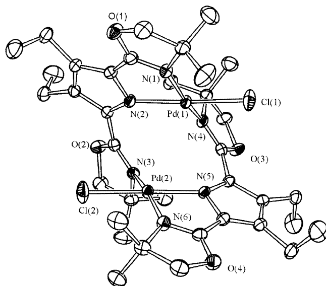
Figure 2. Molecular structure of the palladium complex [\text{Pd}_2\text{Cl}_2(\text{Et}_2\text{dmoxp})_2] ( 7 ); selected bond lengths [Å] and angles [°]: Pd(1)–N(1) 2.031(2), Pd(2)–N(3) 2.043(2), Pd(1)–Cl(1) 2.2922(7), Pd(1)–N(2) 2.036(2), Pd(2)–N(5) 2.031(2), Pd(2)–Cl(2) 2.0311(7), Pd(1)–N(4) 2.035(2), Pd(2)–N(6) 2.036(2); N(1)–Pd(1)–Cl(1) 94.94(6), N(6)–Pd(2)–Cl(2) 95.75(6), N(1)–Pd(1)–N(2) 80.01(8), N(3)–Pd(2)–N(5) 94.48(8), N(2)–Pd(1)–N(4) 96.80(8), N(5)–Pd(2)–N(6) 79.86(8), N(2)–C(7)–C(14)–N(3) 21.4(5), N(4)–C(21)–C(24)–N(5) 28.3(5).
