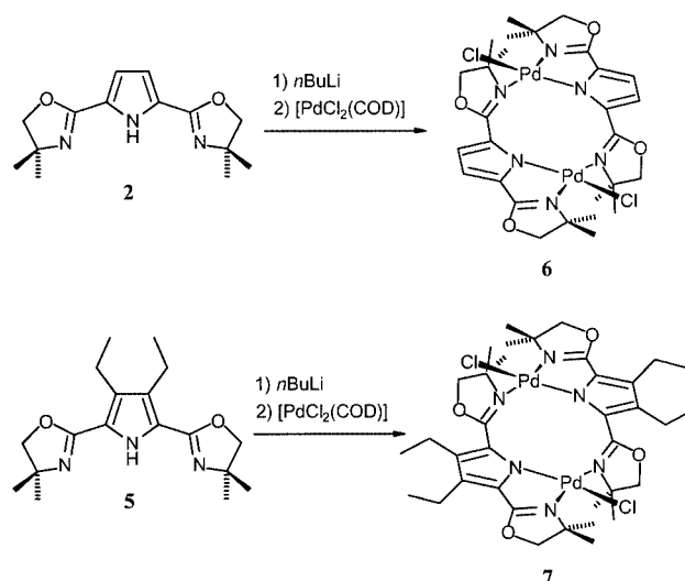
Scheme 2. Synthesis of the helical dinuclear palladium complexes [\text{Pd}_2\text{Cl}_2(\text{dmoxp})_2] ( 6 ) and [\text{Pd}_2\text{Cl}_2(\text{Et}_2\text{dmoxp})_2] ( 7 )
