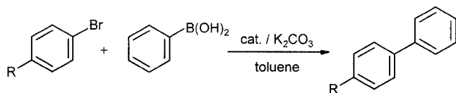
Scheme 7. Suzuki coupling between bromobenzene derivatives and phenylboronic acid
