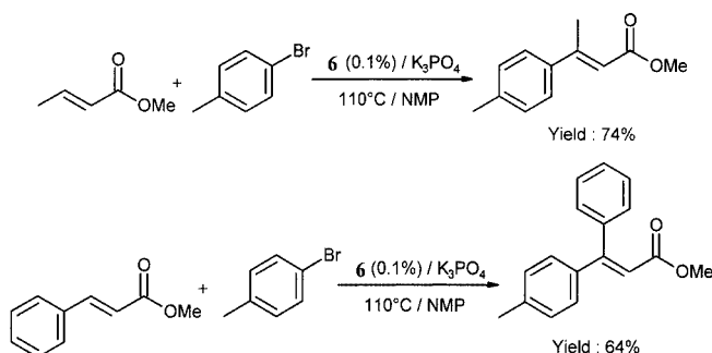
Scheme 5. Heck reactions giving trisubstituted alkenes
