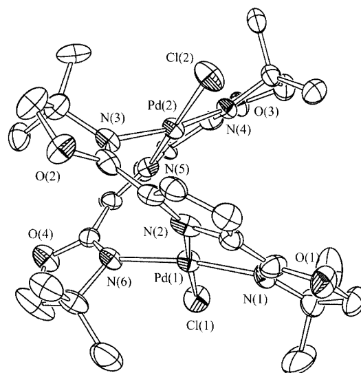
Figure 1. Molecular structure of the palladium complex [\text{Pd}_2\text{Cl}_2(\text{dmoxp})_2] ( 6 ); selected bond lengths [Å] and angles [ ^\circ ]: Pd(1)–N(1) 2.052(8), Pd(1)–N(2) 2.039(8), Pd(1)–N(6) 2.036(8), Pd(1)–Cl(1) 2.296(3), Pd(2)–Cl(2) 2.287(3), Pd(2)–N(3) 2.043(8), Pd(2)–N(4) 2.025(7), Pd(2)–N(5) 2.039(8); N(2)–Pd(1)–N(6) 97.7(3), N(1)–Pd(1)–N(2) 79.8(3), Cl(1)–Pd(1)–N(1) 96.5(2), N(3)–Pd(2)–N(5) 97.7(3), N(4)–Pd(2)–N(5) 79.9(3), N(2)–C(28)–C(8)–N(3) 29.3(5), N(5)–C(19)–C(22)–N(6) 26.4(5)
