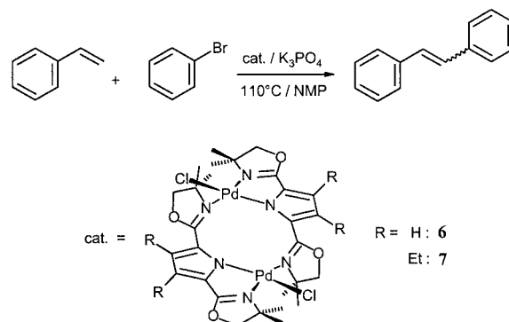
Scheme 3. Application of the palladium complexes [\text{Pd}_2\text{Cl}_2(\text{dmoxp})_2] ( 6 ) and [\text{Pd}_2\text{Cl}_2(\text{Et}_2\text{dmoxp})_2] ( 7 ) in the Heck reaction between bromobenzene and styrene
